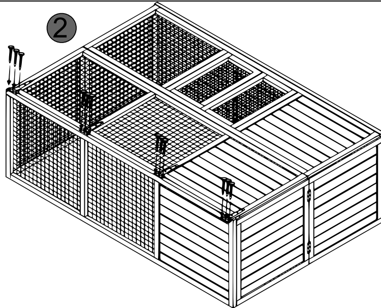
Steg 2 | A 30×16 (12)
