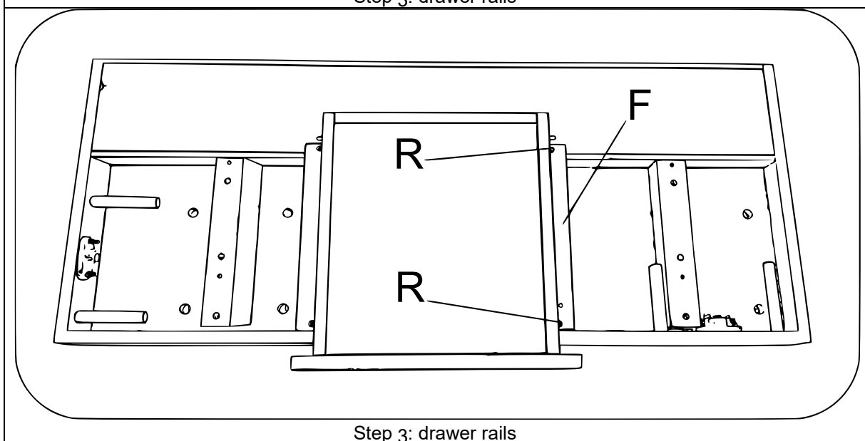
Step 3: drawer rails
