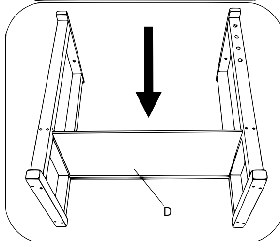
Step 1: worktop and legs
